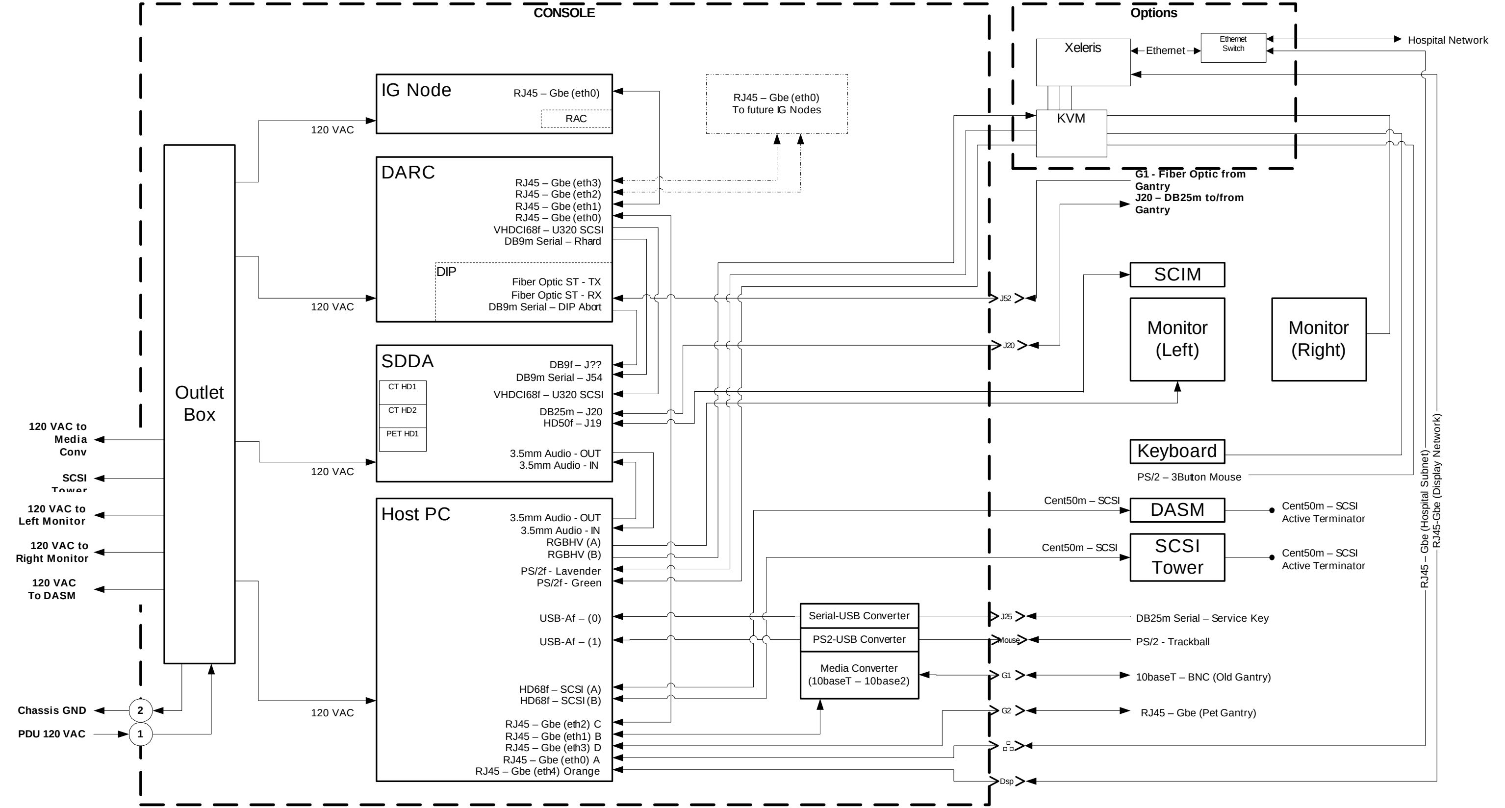
DST_HP60 Console Block Diagram
